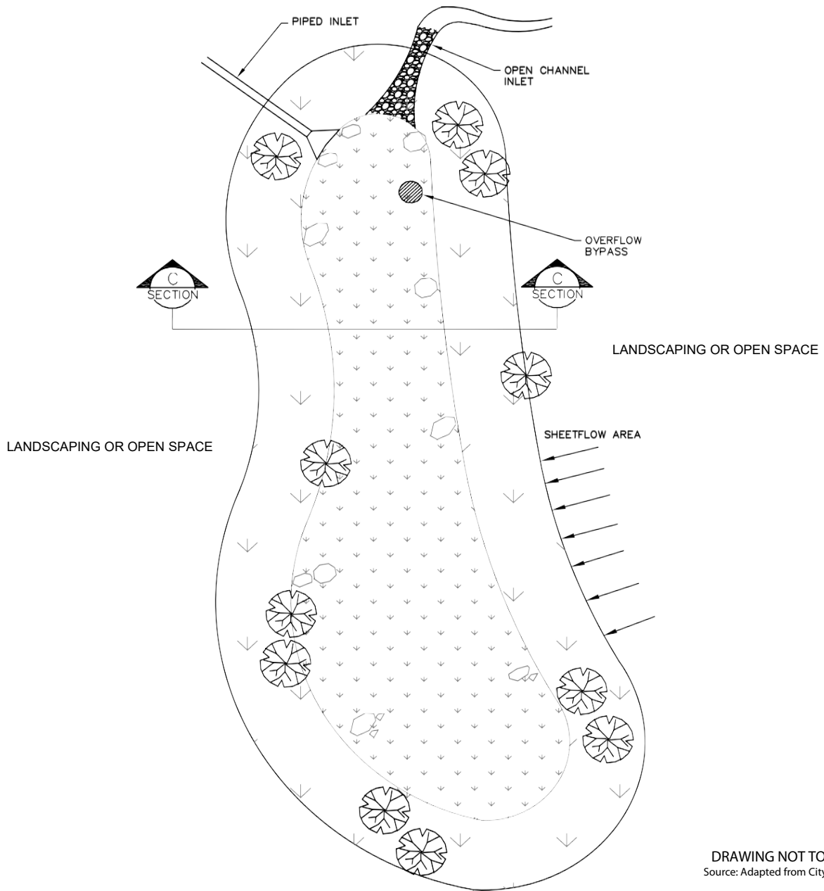
BIORETENTION IN LANDSCAPE OR OPEN SPACE AREAS Plan View
