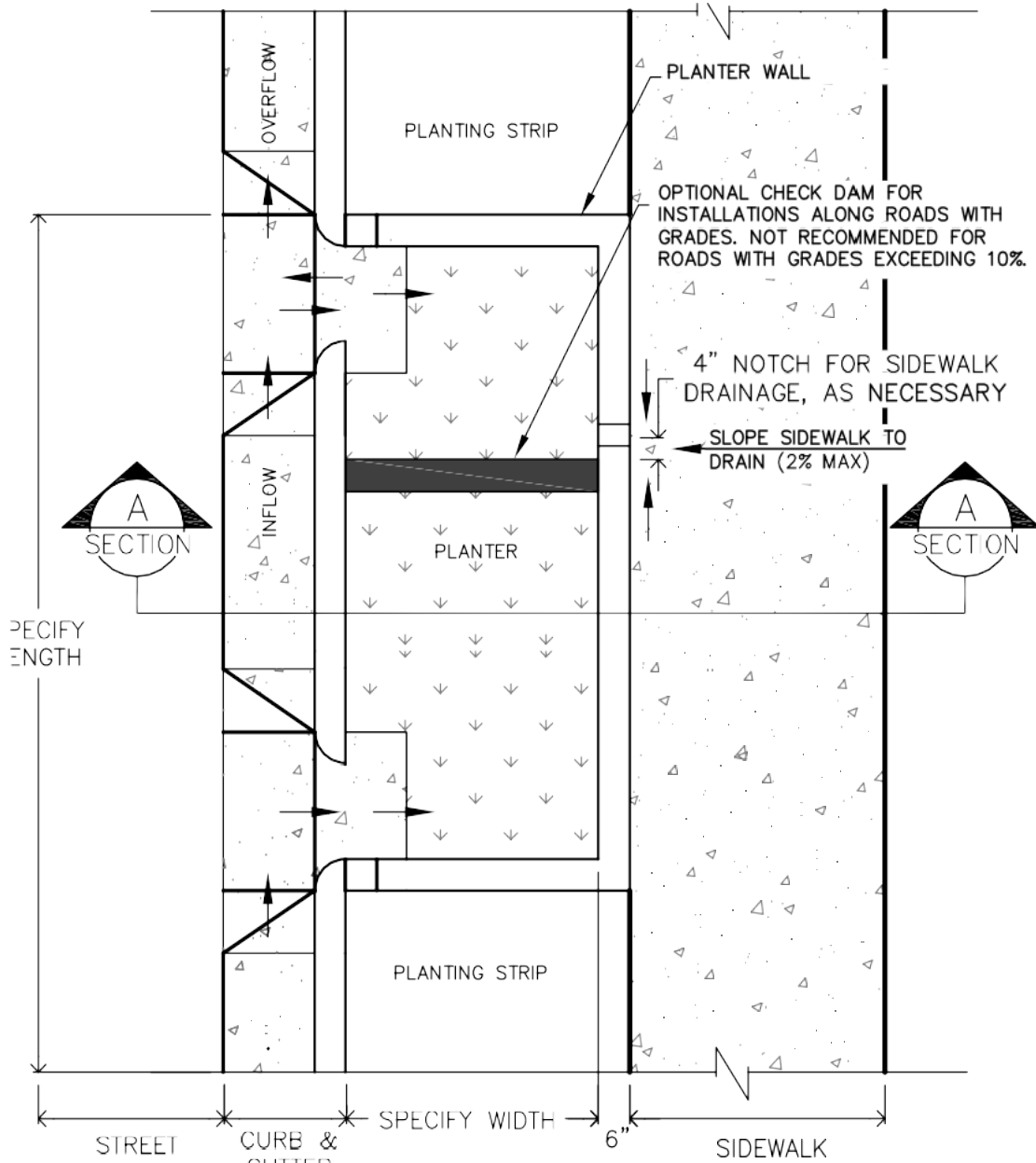
IN STREET BIORETENTION – WITHOUT PARKING Plan View
